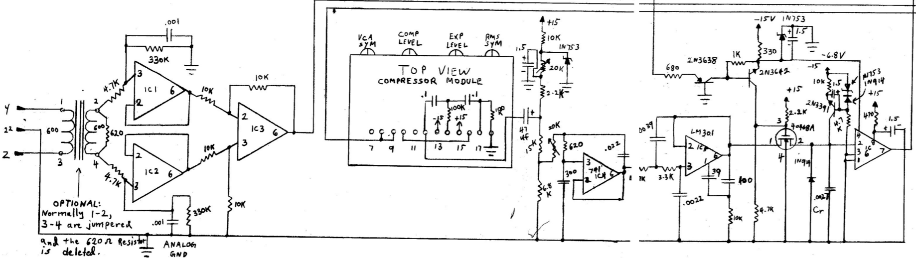
1745M INPUT AND TIMING BOARD M691
